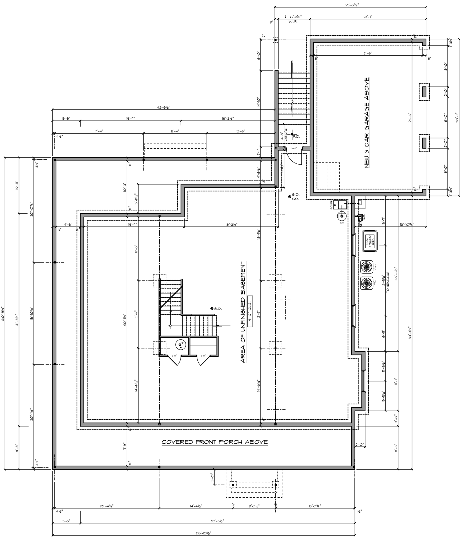
FOUNDATION - BSMT. PLAN
